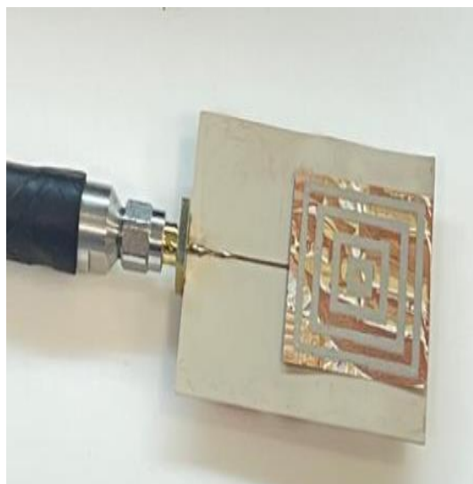
Figure19. Near field RFID tag identification printed on Egyptian banknote by using a wideband antenna.
